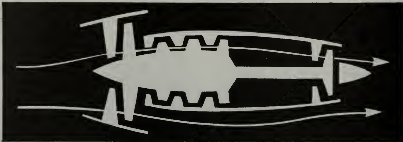
FIGURE 2-25. Airflow through a forward-fan engine.
